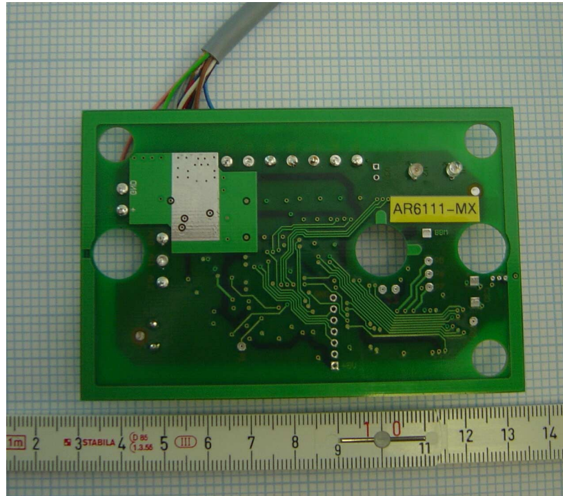
Bottom view of printed board
