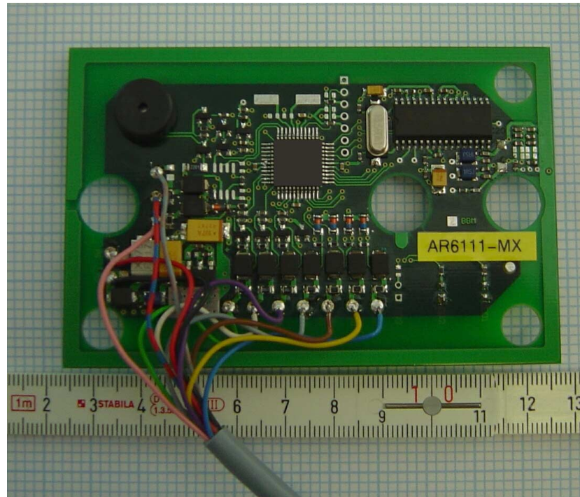
Top view of printed board
