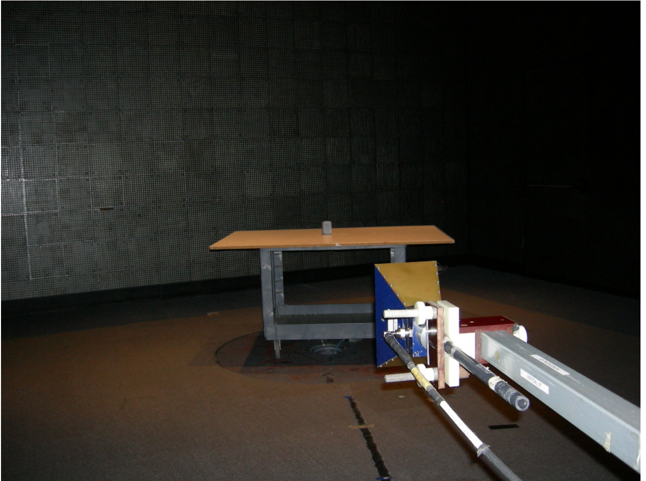
Figure 1: Radiated Emissions
