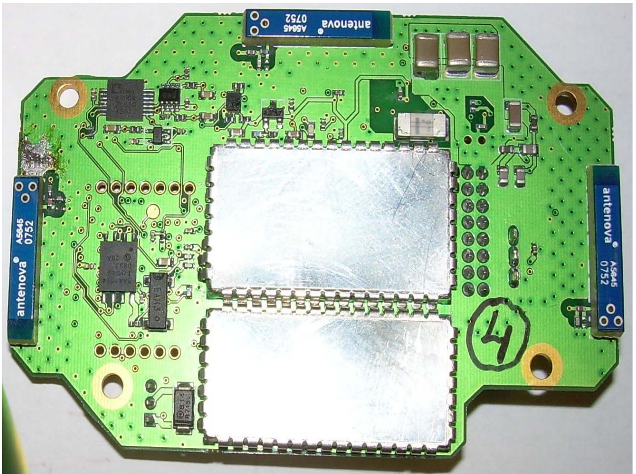
Figure 1: PCB Front
