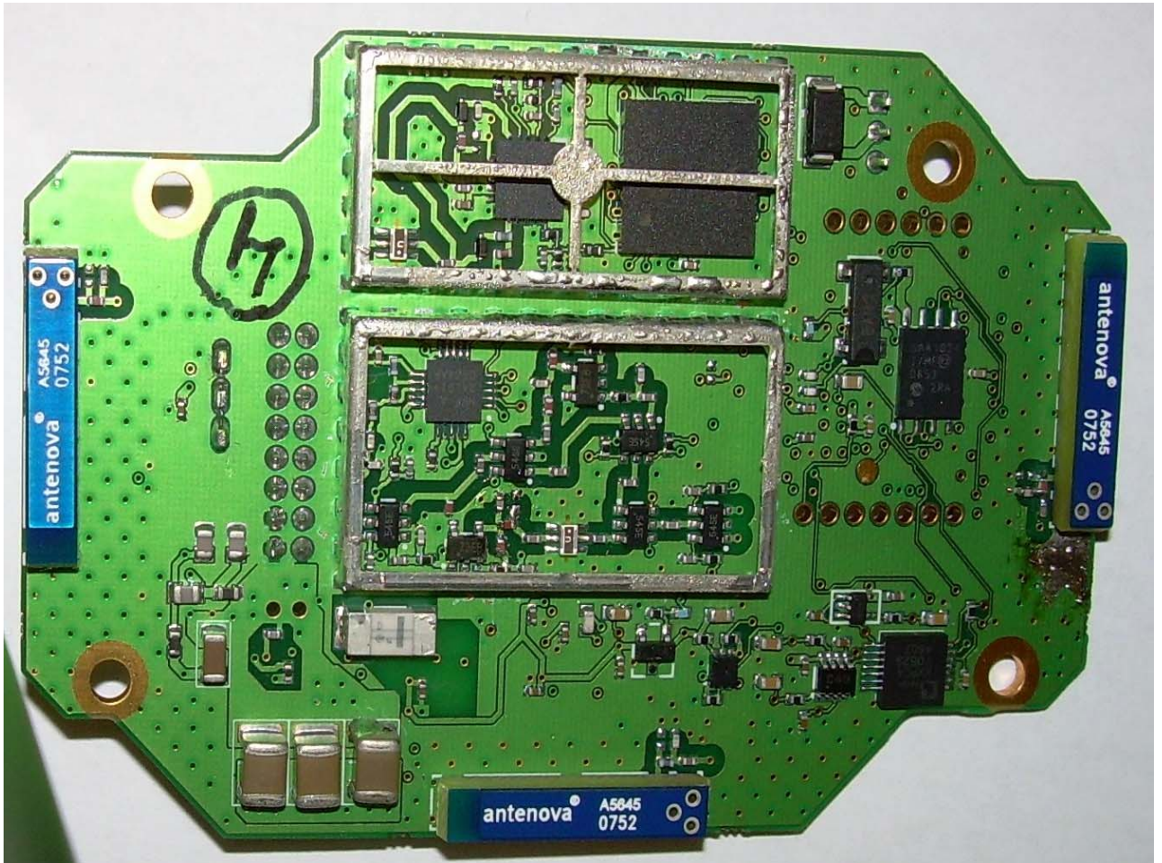
Figure 2: PCB Front (Shields Removed)
