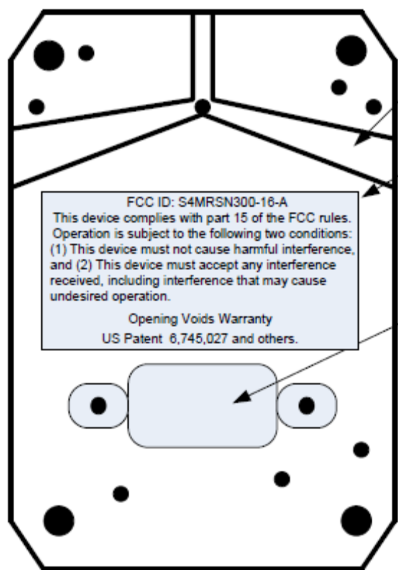
RSN300 UNIT LABELING BOTTOM
