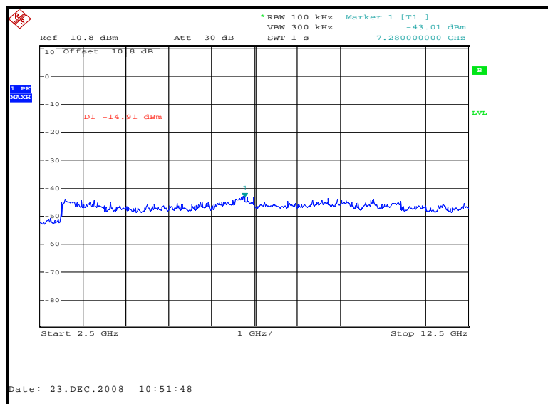
Figure 7.6.2.2-8: 2.5 GHz – 12.5 GHz –High Channel
