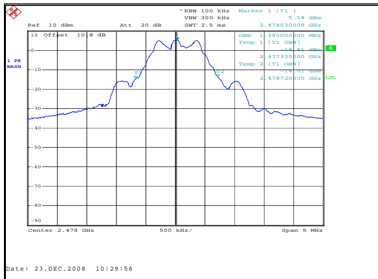
Figure 7.4.2-6: 99% Bandwidth Plot – High Channel
