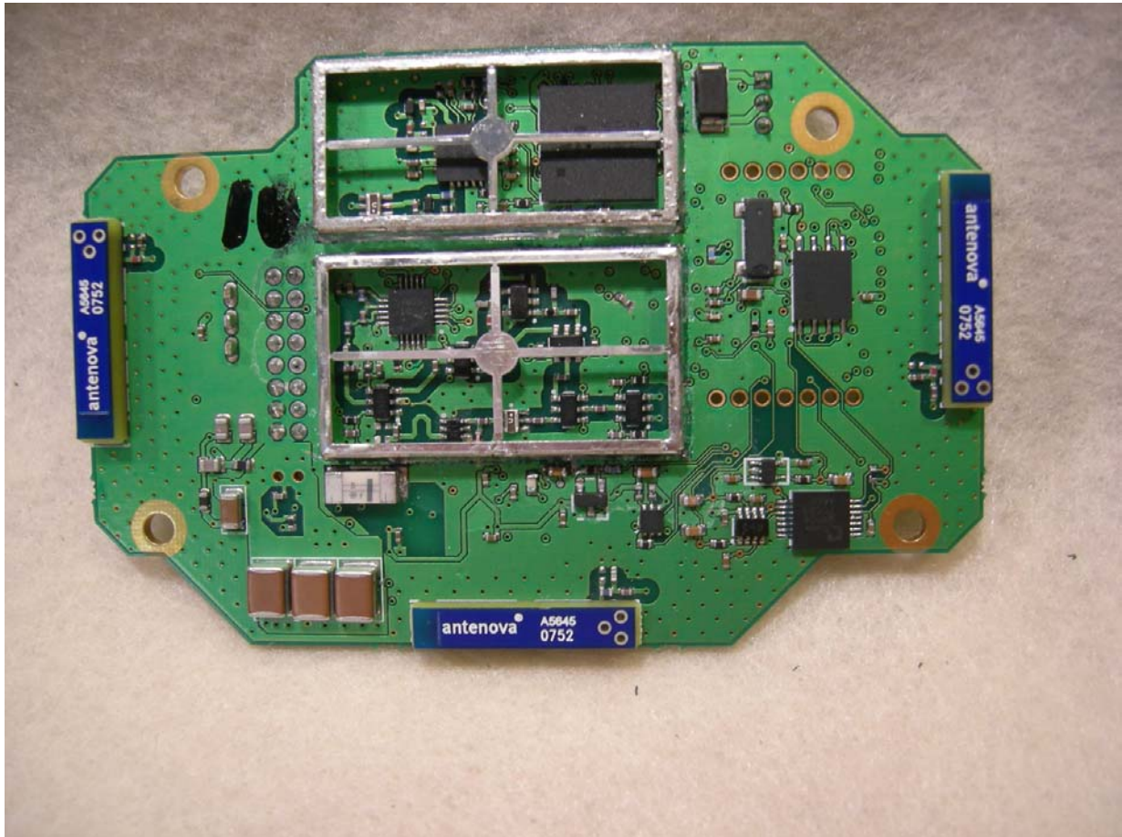
Figure 3: PCB Front (Shields Removed)
