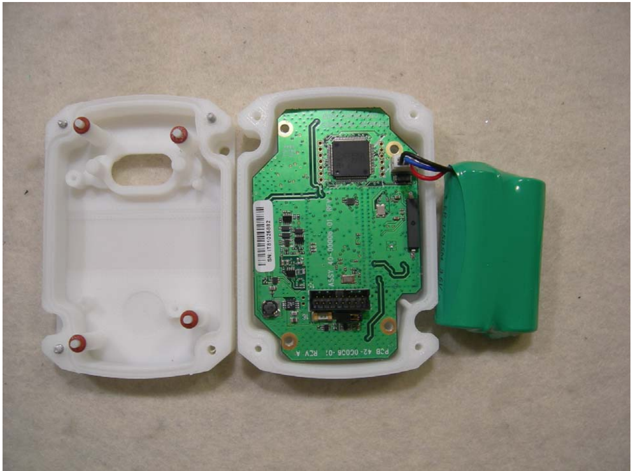
Figure 1: Assembled View
