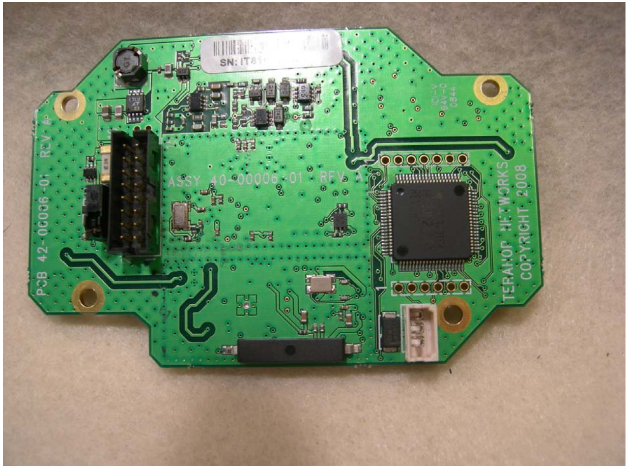
Figure 4: PCB Back
