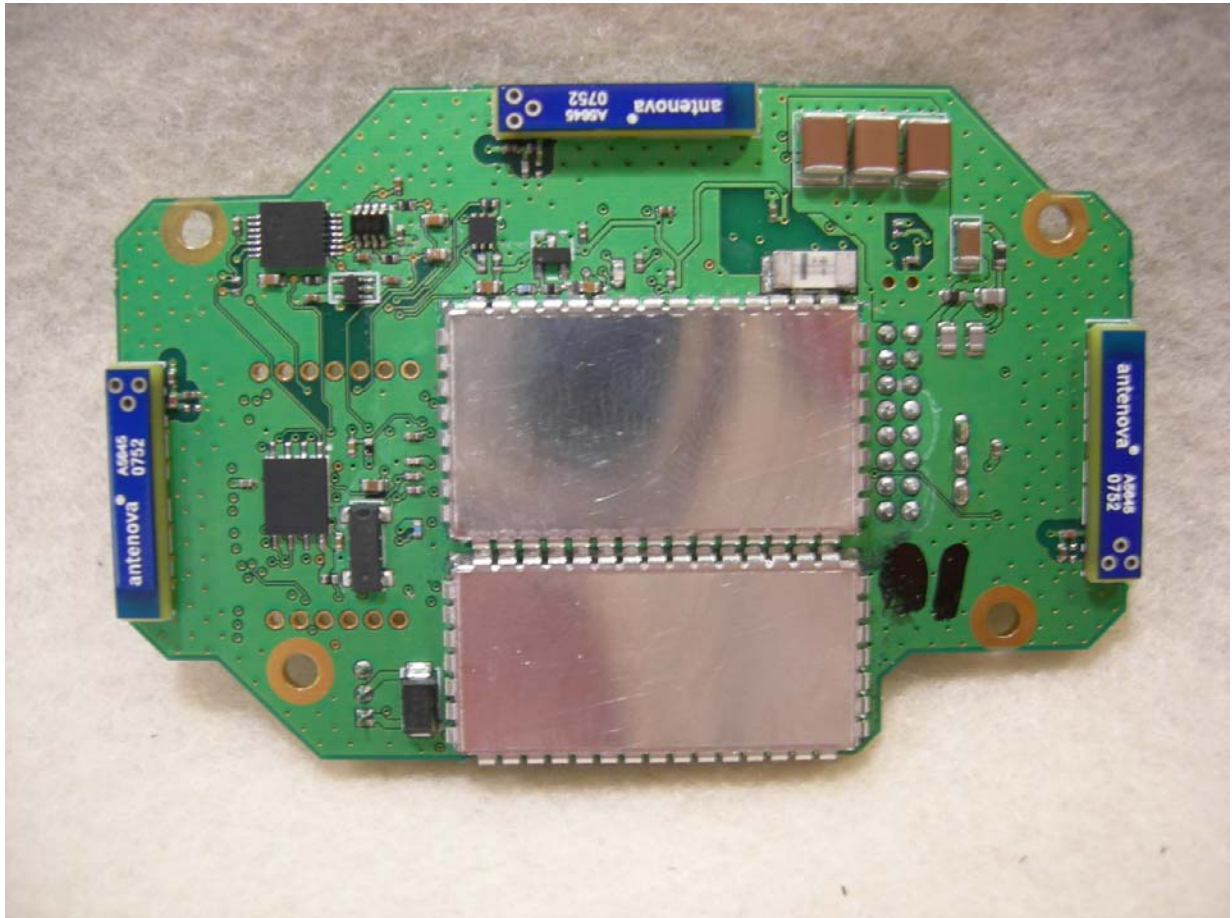
Figure 2: PCB Front
