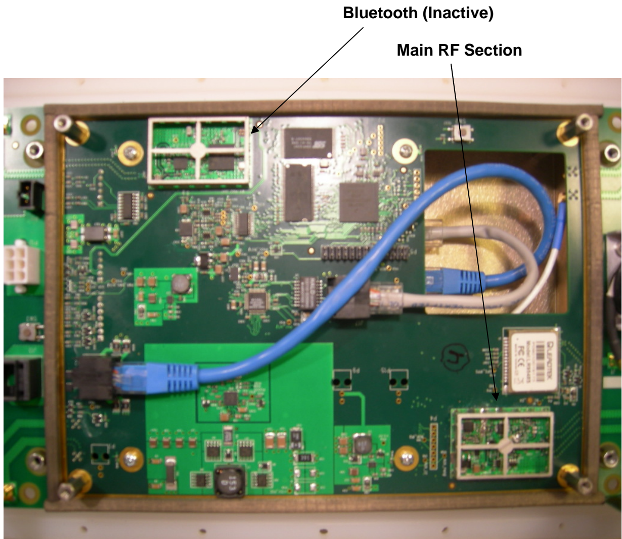
Figure 5: RF Board Front
