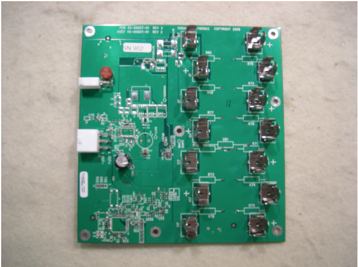
Figure 3: Power Supply Board Front
