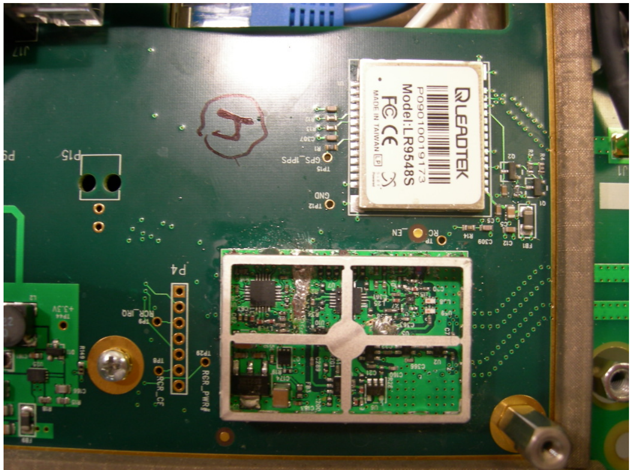
Figure 6: RF Board (RF Section)
