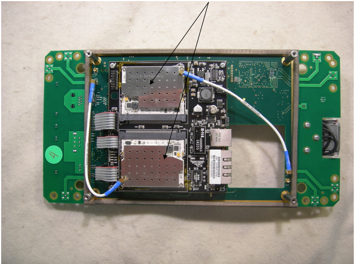
Figure 7: RF Board Back w/ 802.11a Backhaul radio boards
