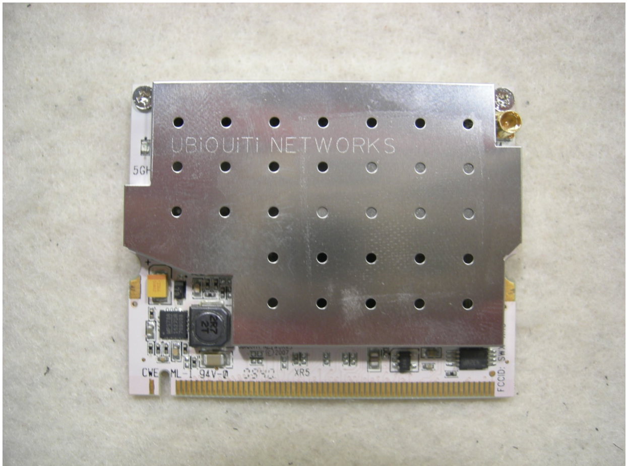
Figure 9: Modular Approved 802.11a Radio (FCC ID: SWX-XR5)
