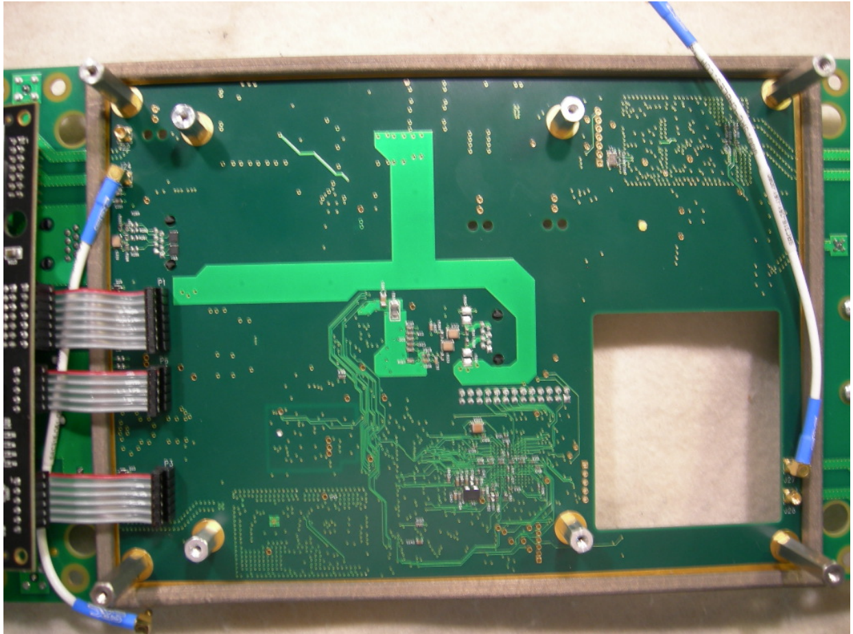
Figure 8: RF Board Back
