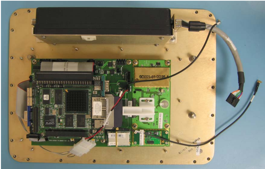
Internal View w/ Electronics Cover Removed
