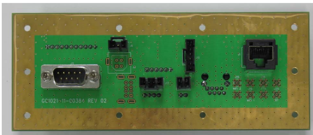
Bottom View
