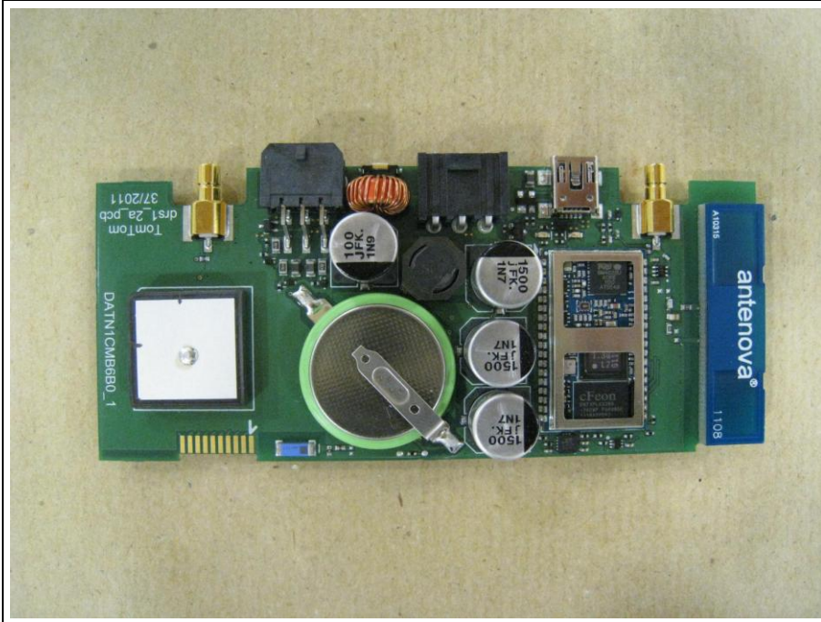
EUT PCB TOP WITHOUT SHIELDINGS
