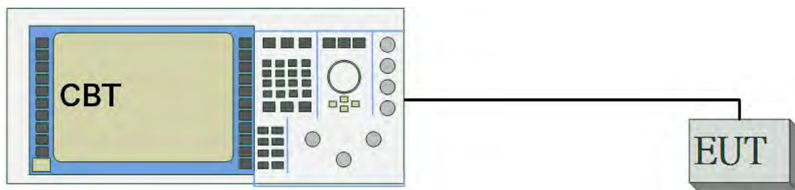
Fig. 2-2 C Conducted (Antenna Port) Configuration
