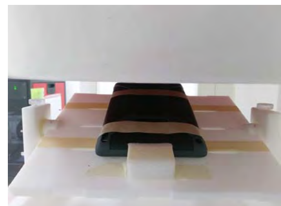
Fig.4 EUT Back side_curve to flat phantom
