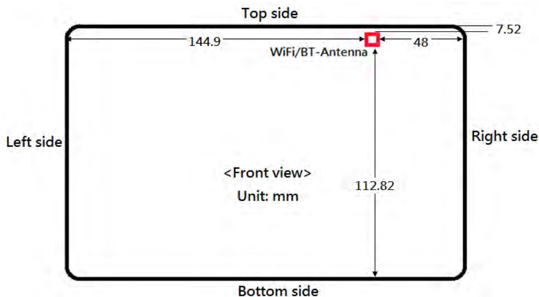
Fig.7 Antenna position of EUT
