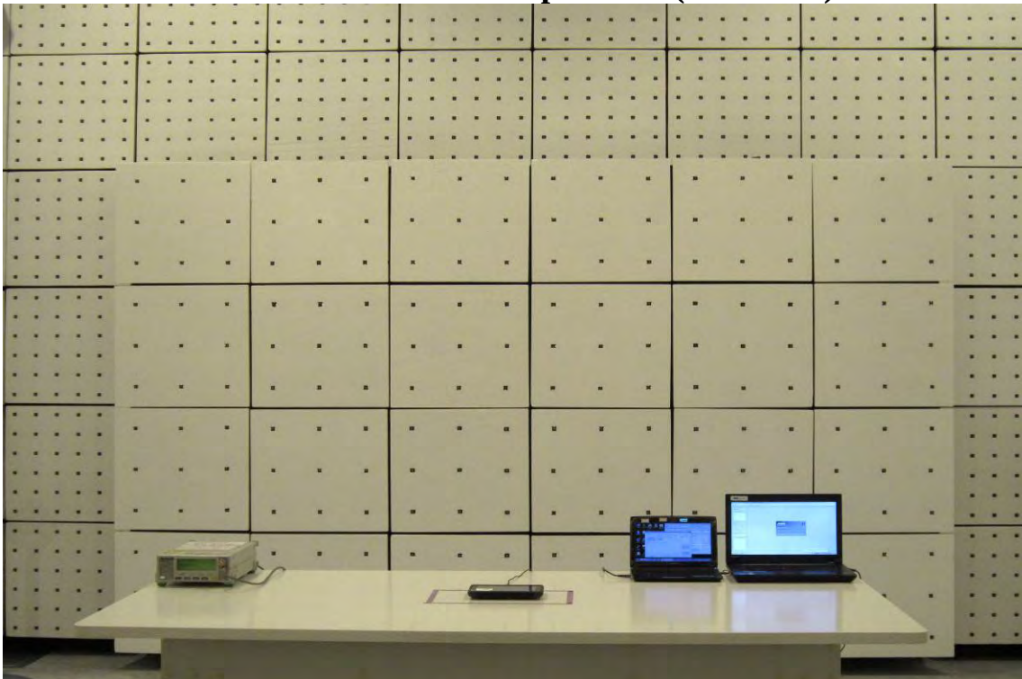
Radiated Emission Set up Photos (E2 PLAN)
