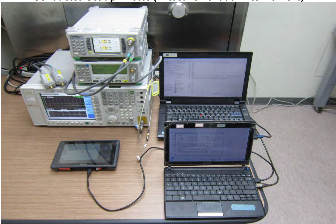
Conducted Set up Photos (Measurement at Antenna Port)
