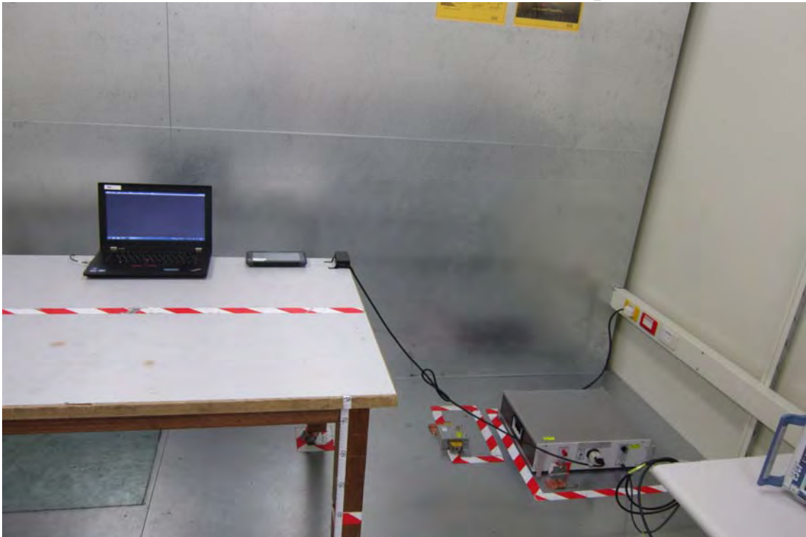
AC Power-line Conducted Emission Set up Photo
