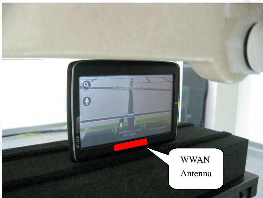
Fig.6 Body worn_Right side to flat phantom
