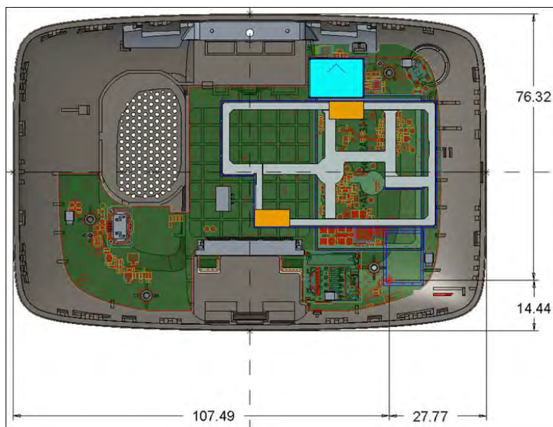
Fig.11 antenna location
