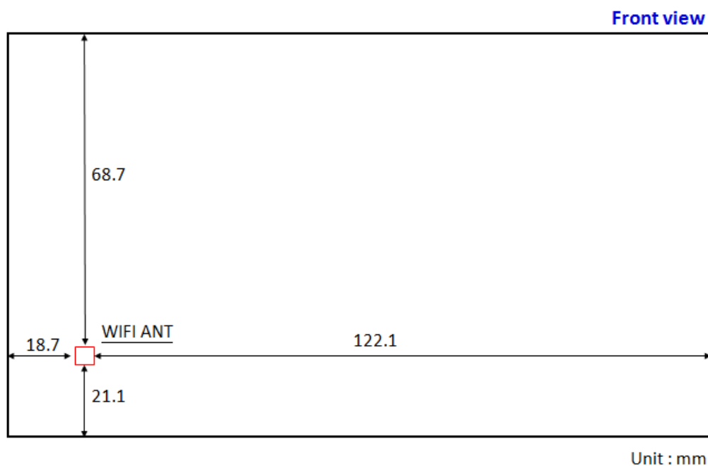
Antenna location (front view)
