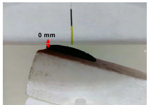
Fig.8 EUT Back side_curve (0mm) to flat phantom
