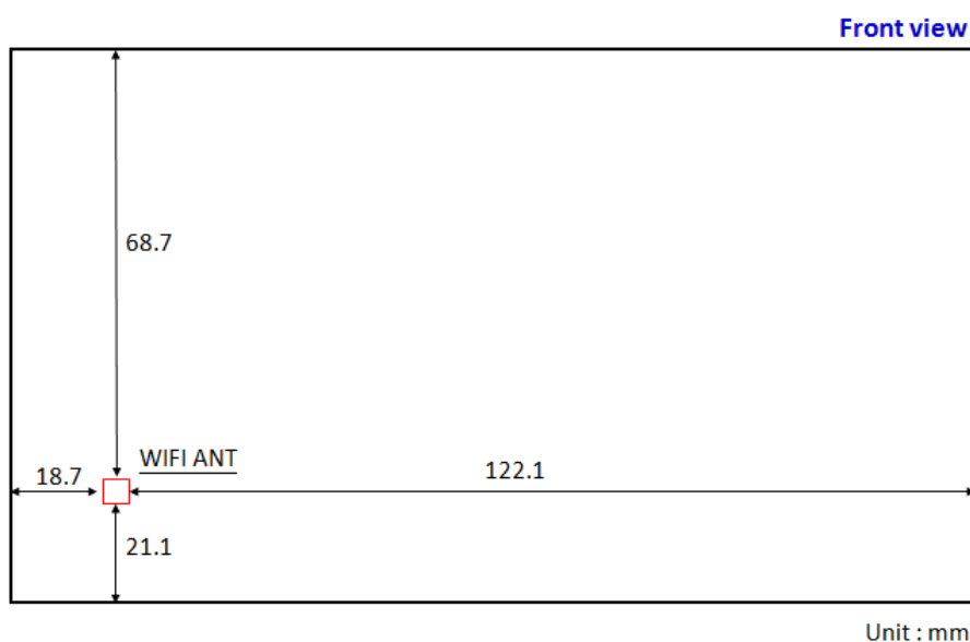
Fig.14 Antenna location (front view)
