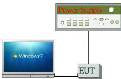
Fig 2-2 Conducted (AC power line) Configuration
