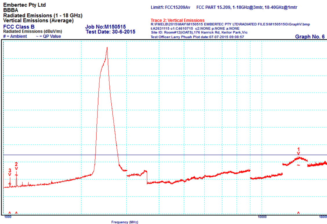
Graph 6: Vertical Polarity (average) 1 – 18 GHz
