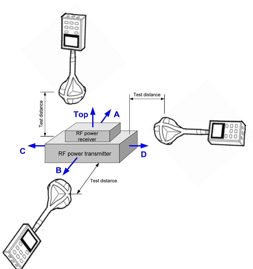
Figure 7.1.1 Setup for RF exposure measurements
