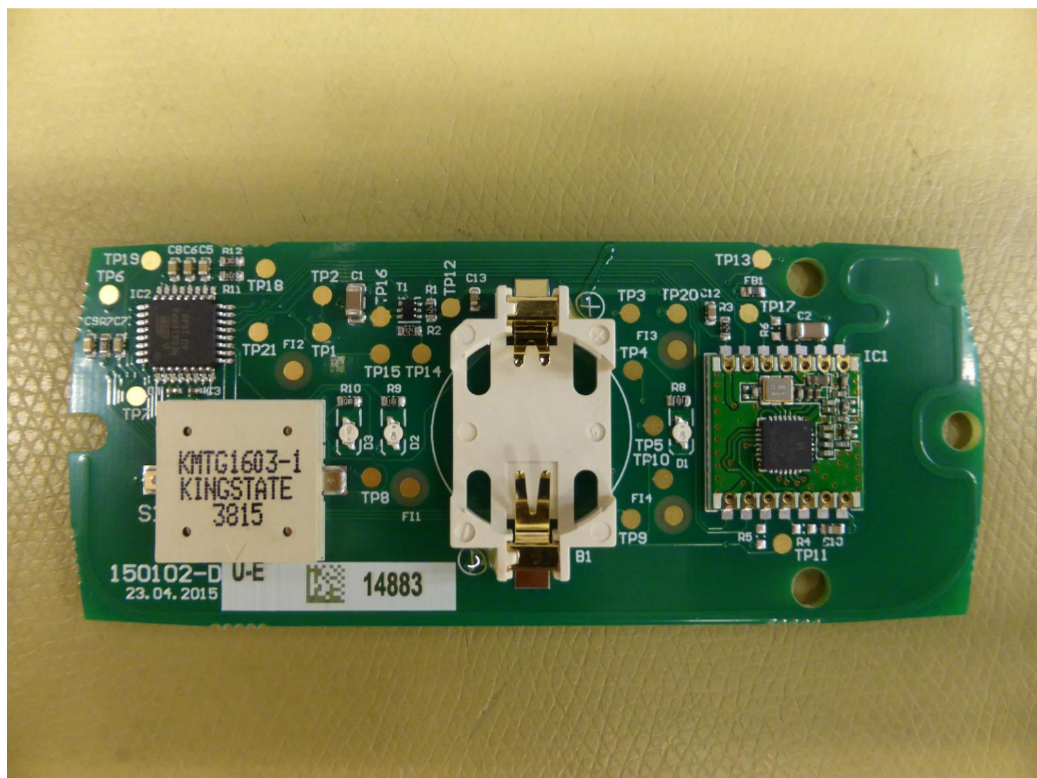
RCT-2U/150102 Internal Photo TOP
