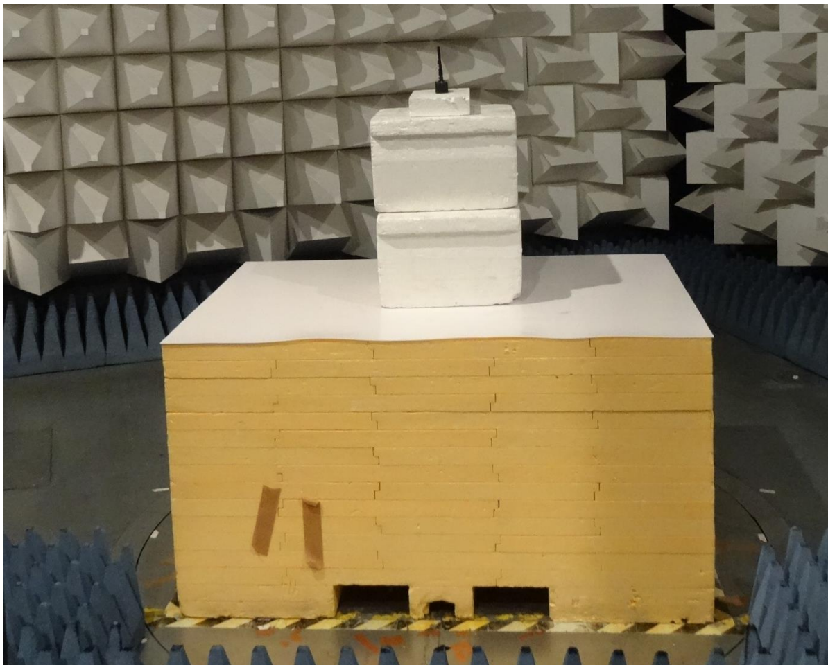
Radiated emission setup over 1GHz
