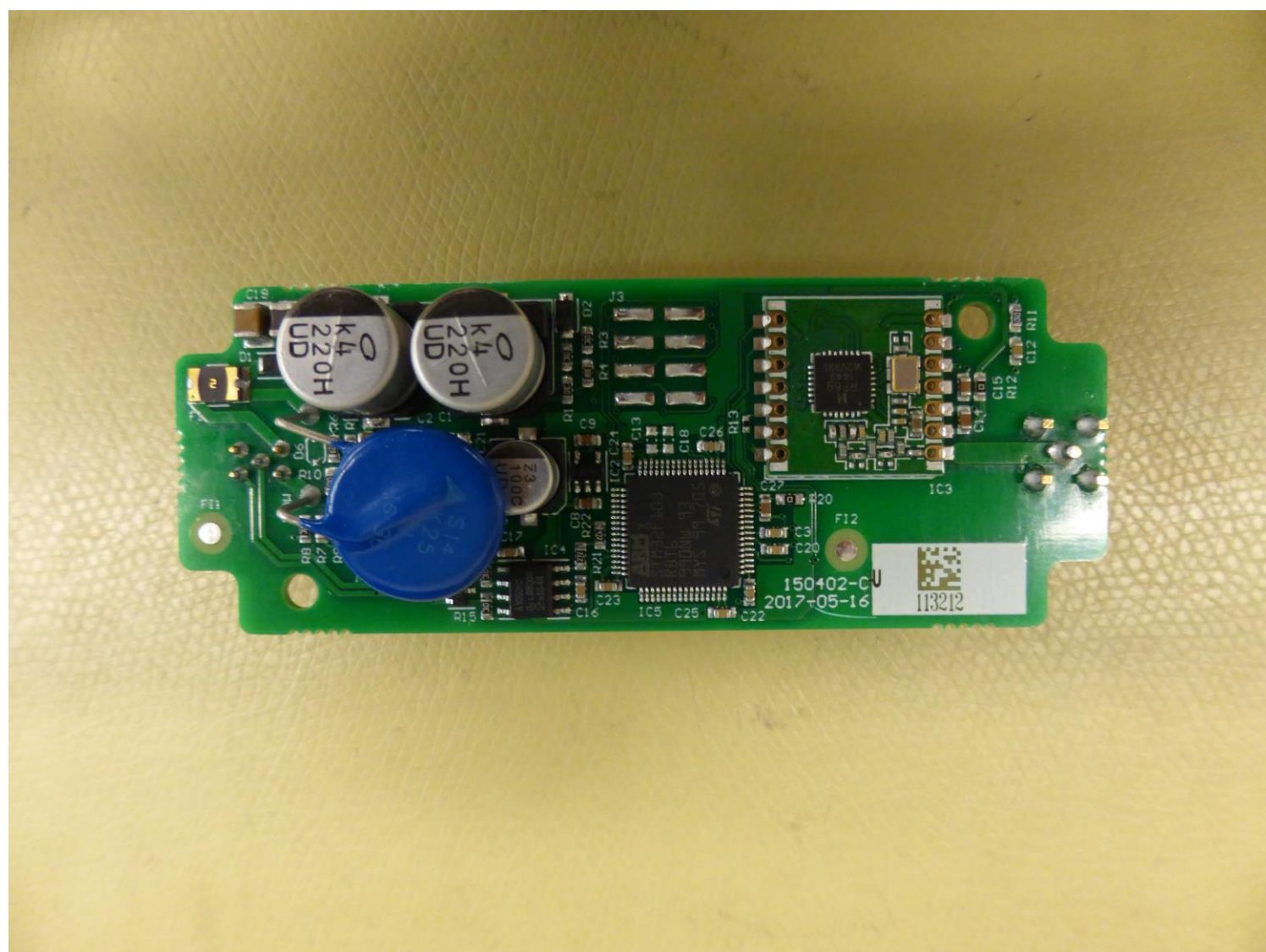
RCRS-2U/150402 Internal Photo BOTTOM
