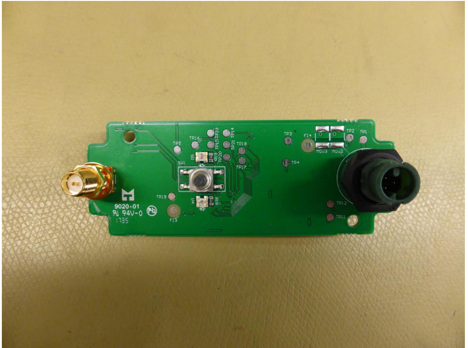
RCRS-2U/150402 Internal Photo TOP
