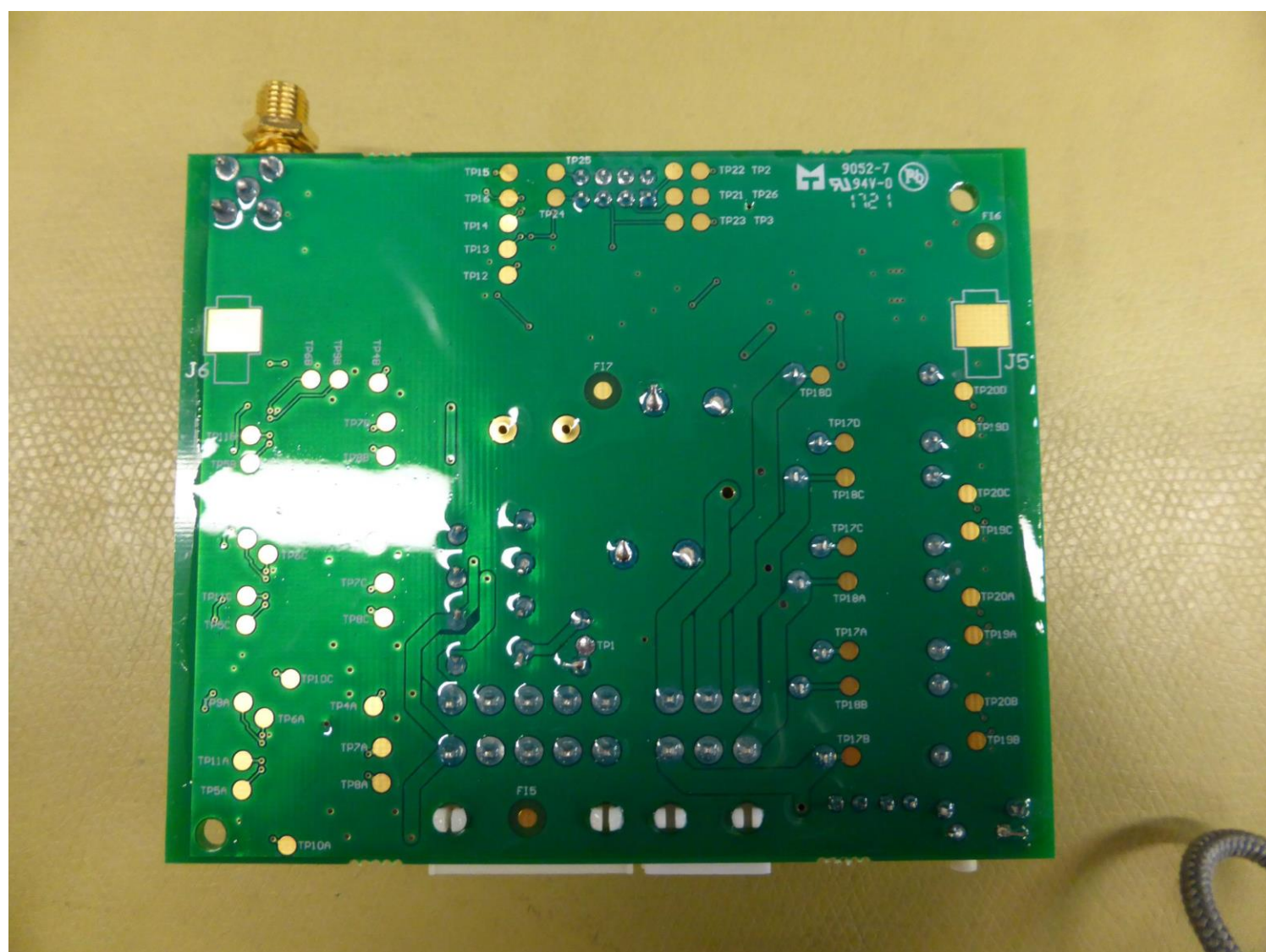
RCR-2U/150701 Internal Photo BOTTOM
