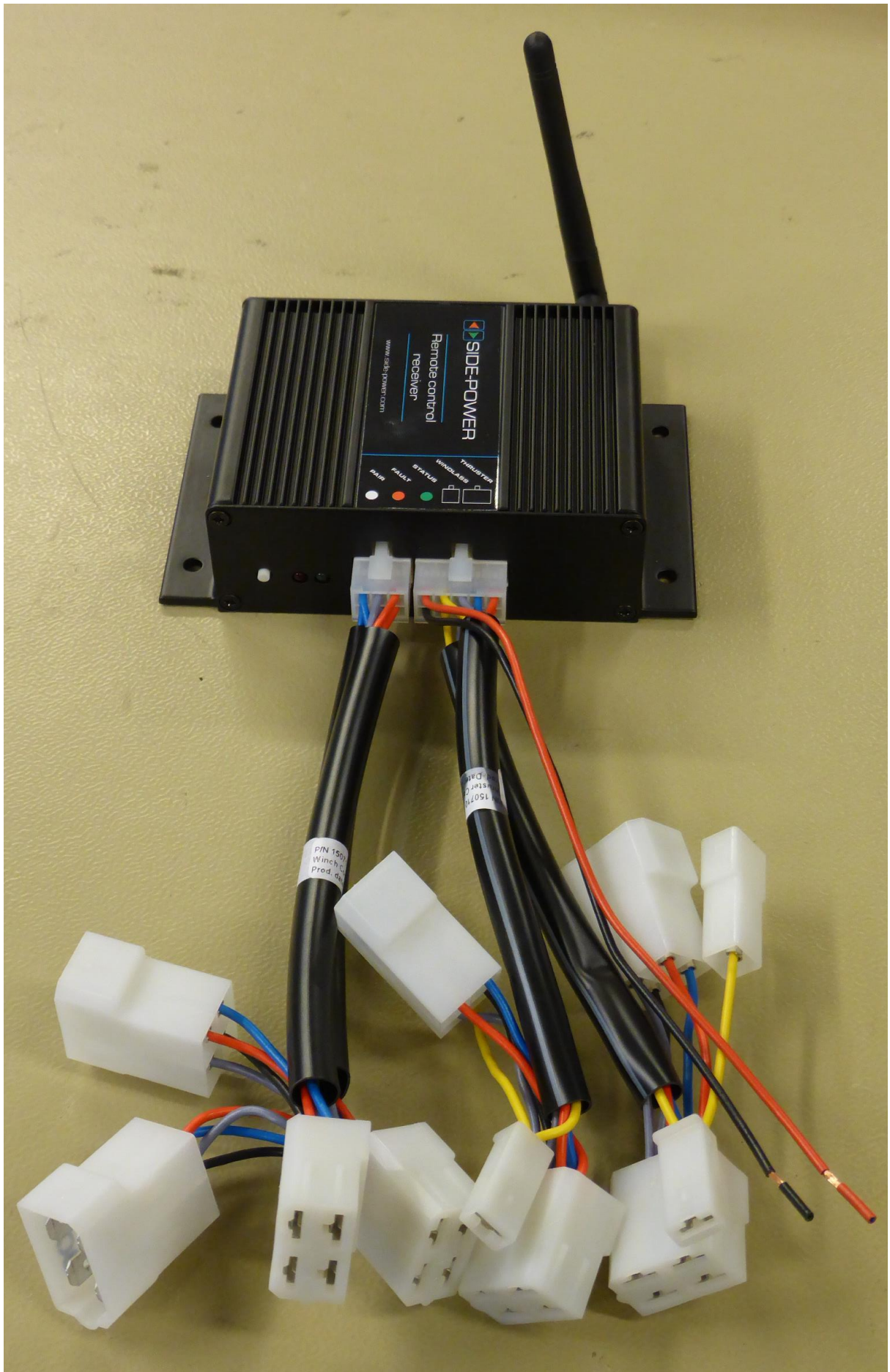
RCR-2U External Photo TOP-RIGHT with connector harness attached
