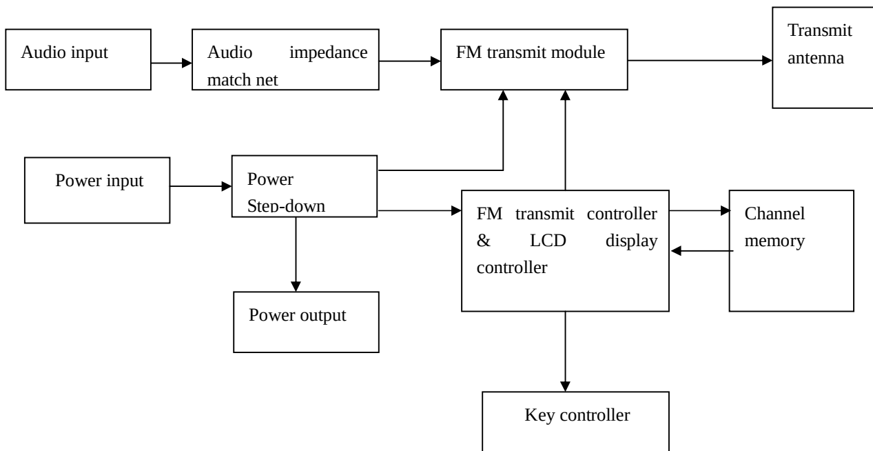
KC-9502/P-25 logic drawing
