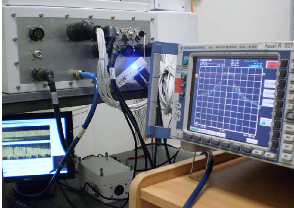
Conducted Spurious at Antenna Port
