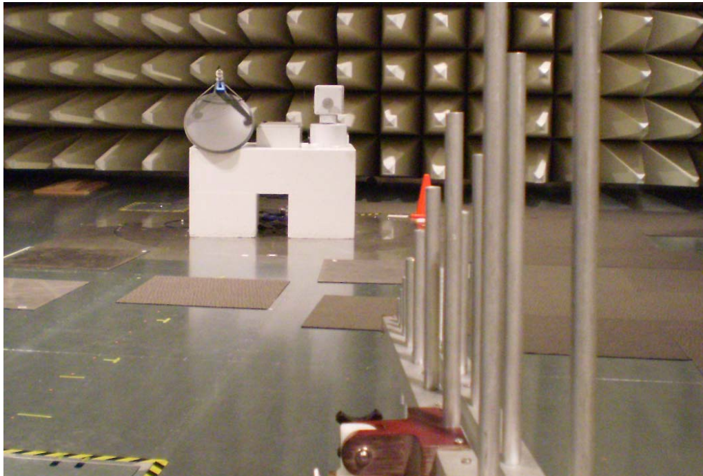
Radiated Emissions below 1 GHz
