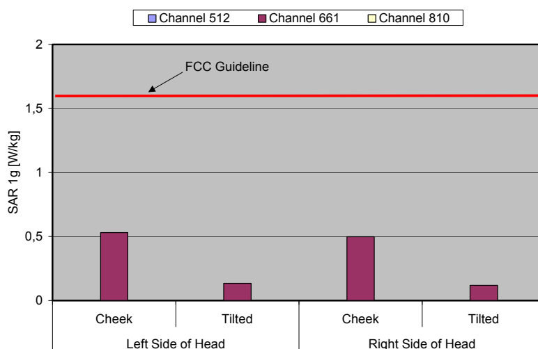
Fig. 8: The measured head phantom SAR values for the FL Telecom ApS O2 XM for PCS 1900 in comparison to the FCC exposure limit.
