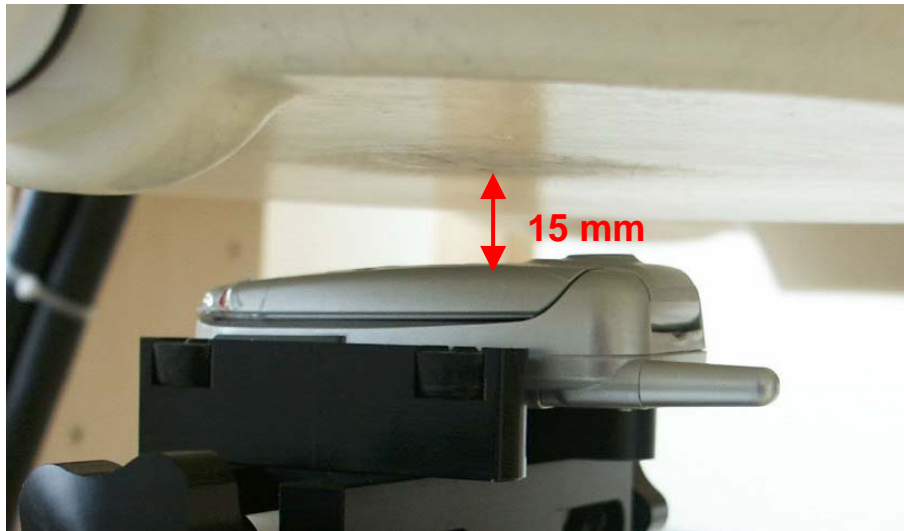
Fig. 22: Body worn configuration, GPRS (Class 10), antenna towards the ground.
