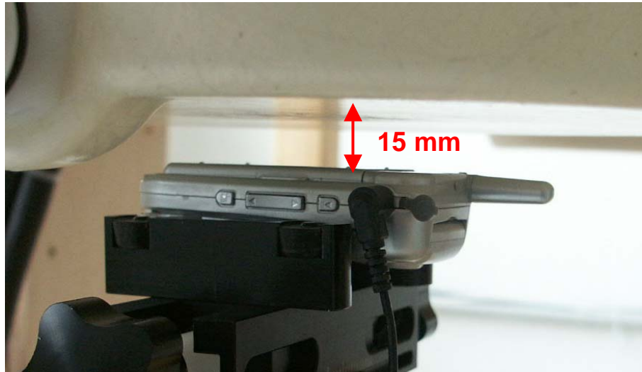
Fig. 20: Body worn configuration, GSM with headset, antenna towards the phantom.
