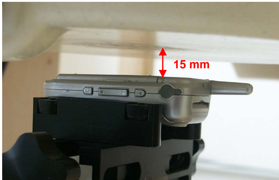
Fig. 21: Body worn configuration, GPRS (Class 10) antenna towards the phantom.
