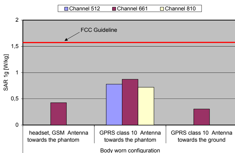
Fig. 9: The measured SAR values in body-worn configuration for the FL Telecom ApS O2 XM for PCS 1900 in comparison to the FCC exposure limit.
