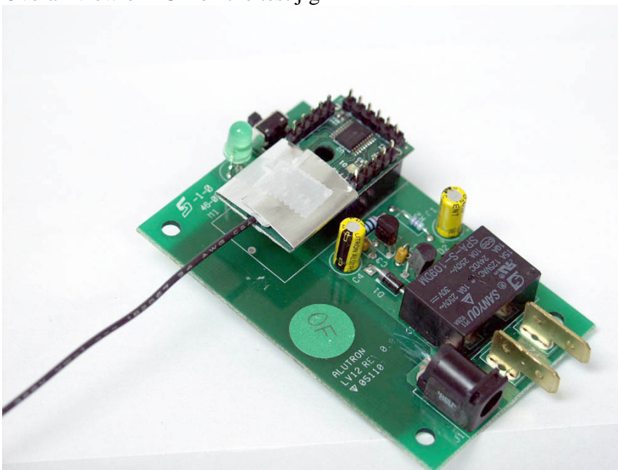
Overall view of EUT on the test jig
