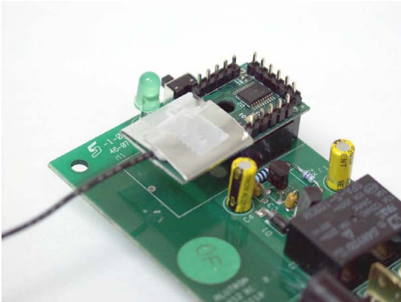
Overall view of EUT on the test jig
