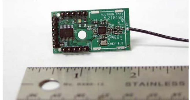
EUT Top View without Shielding
