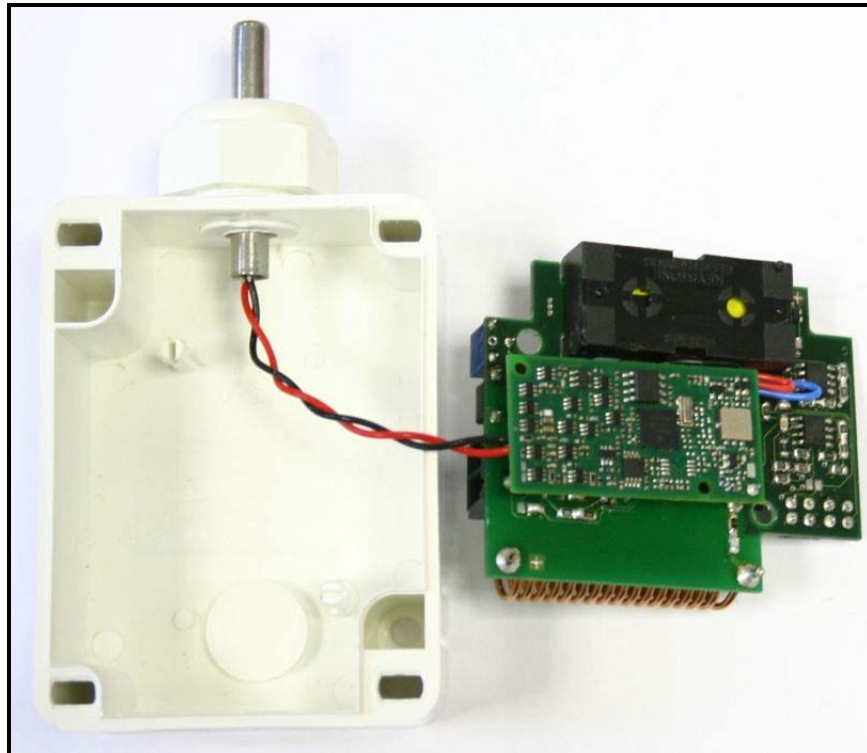
Photograph 5: Inside Front with Radio PCB
