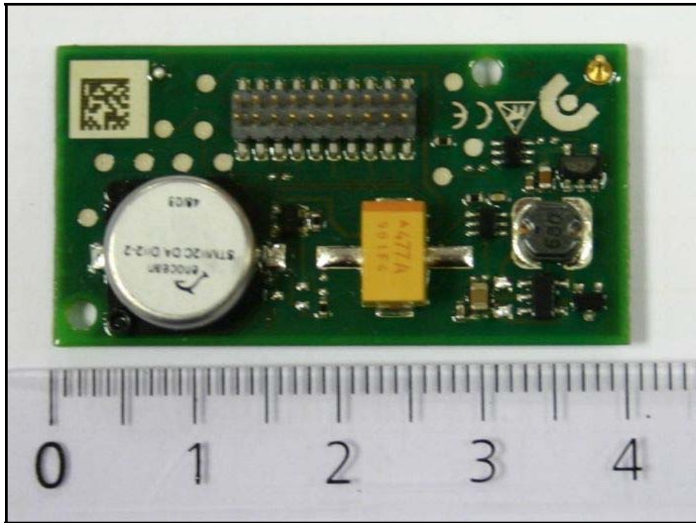
Photograph 7: Back of Radio PCB
