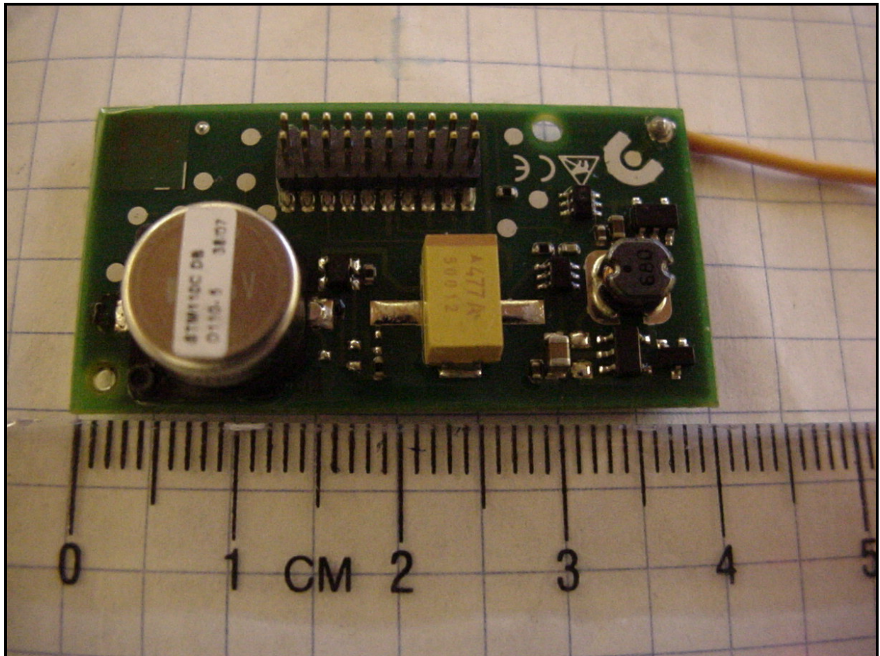
Photograph 7: Back of Radio PCB
