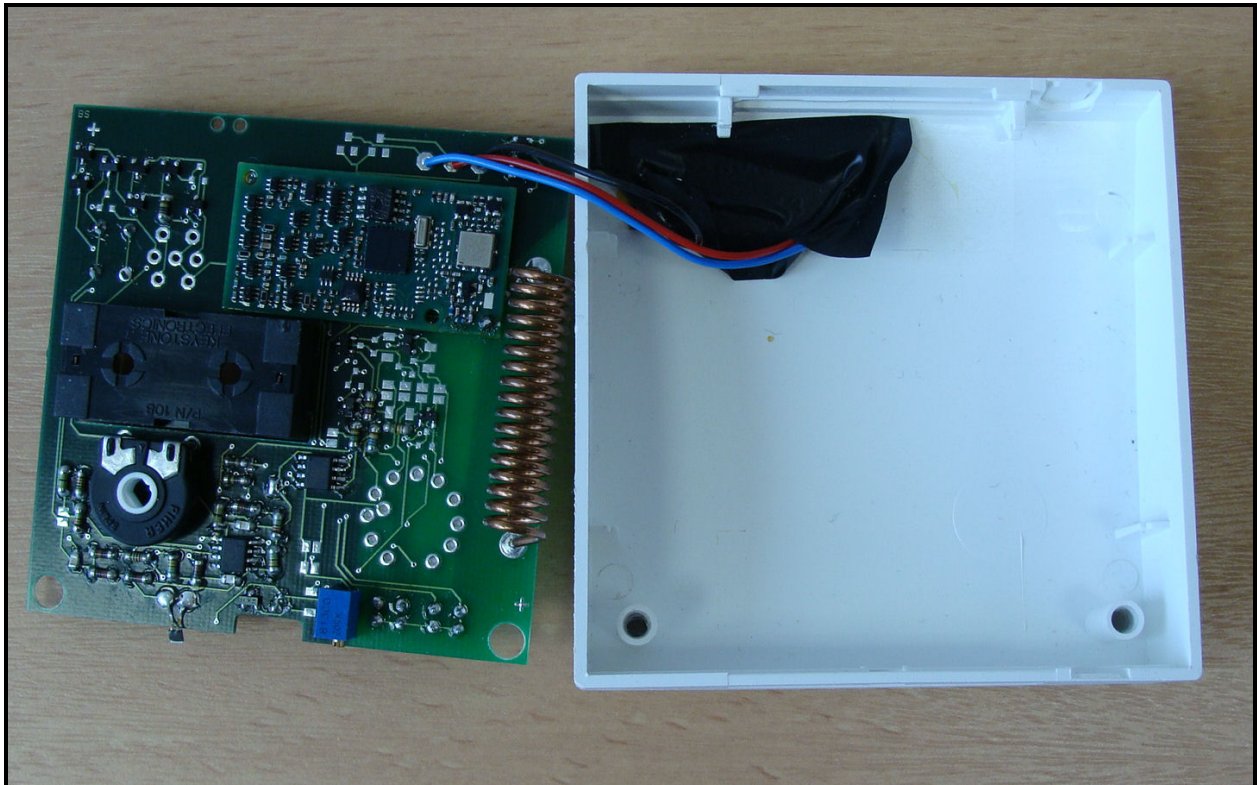
Photograph 5: Inside Front with Radio PCB
