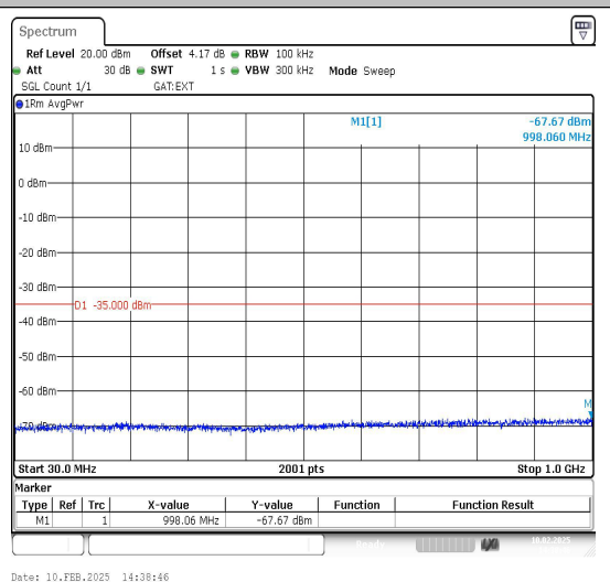
Band41_5MHz_16QAM_41565_1RB#0_30~1000 30~1000
