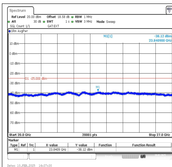
Band41_5MHz_QPSK_41565_1RB#0_20000~27000 000_20000~27000
