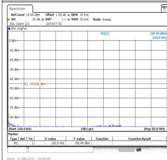
Band41_5MHz_16QAM_41565_1RB#0_0.15~30 _0.15~30
