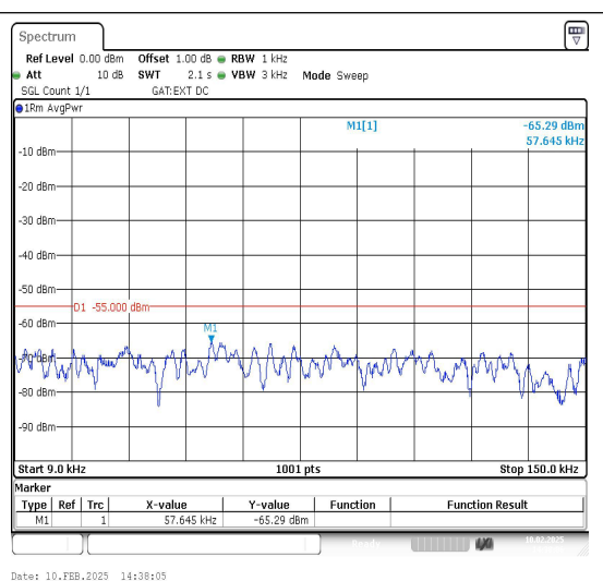
Band41_5MHz_16QAM_41565_1RB#0_0.009~0.1 5_0.009~0.15
