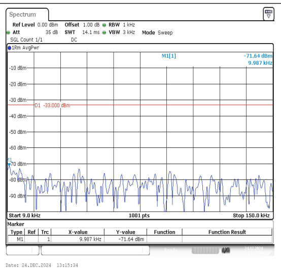
Band26_15MHz_16QAM_26865_1RB#0_0.009~0.15
