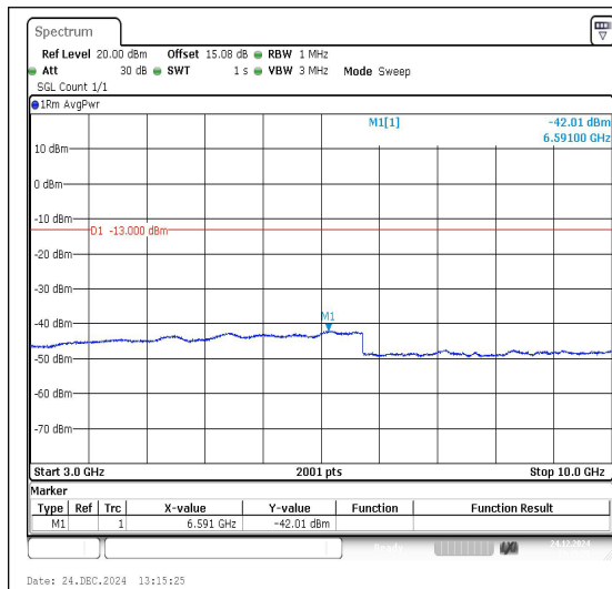
Band26_15MHz_QPSK_26865_1RB#0_3000~10000
