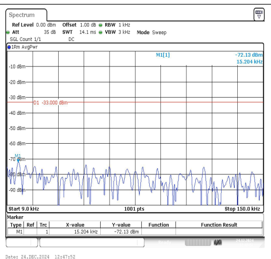
Band26_10MHz_16QAM_26990_1RB#0_0.009~0.15
