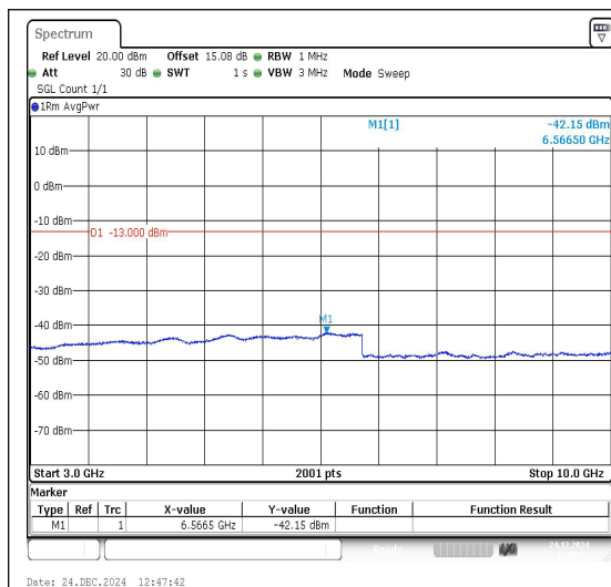
Band26_10MHz_QPSK_26990_1RB#0_3000~10000
