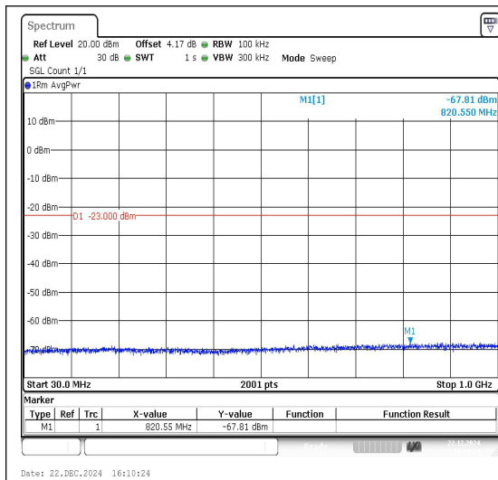
Band25_1.4MHz_QPSK_26683_1RB#0_30~1000_30~1000
