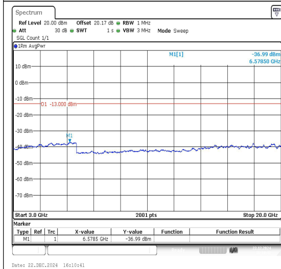
Band25_1.4MHz_QPSK_26683_1RB#0_3000~20000_000_3000~20000
