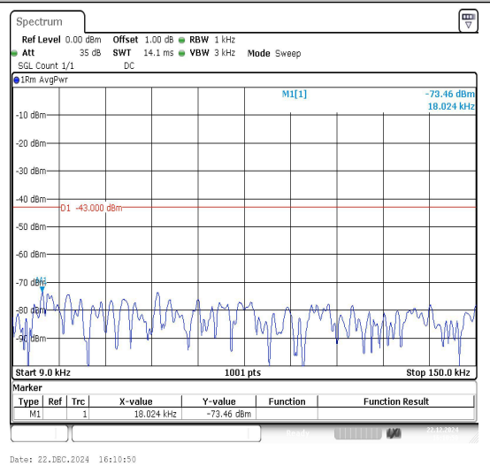
Band25_1.4MHz_16QAM_26683_1RB#0_0.009~0.15_0.009~0.15
