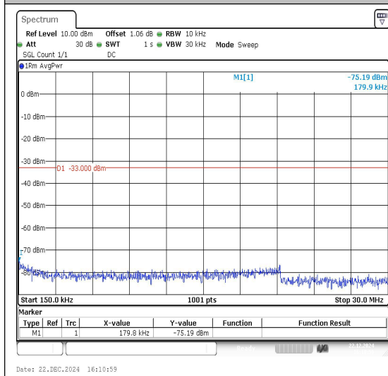
Band25_1.4MHz_QPSK_26683_1RB#0_3000~20000_000_3000~20000
