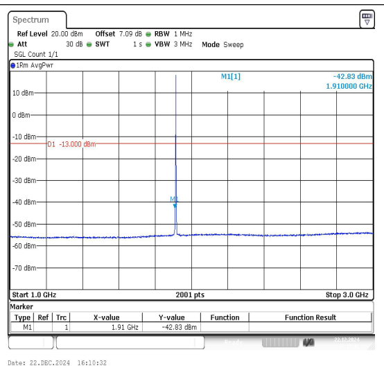
Band25_1.4MHz_QPSK_26683_1RB#0_1000~3000_00_1000~3000
