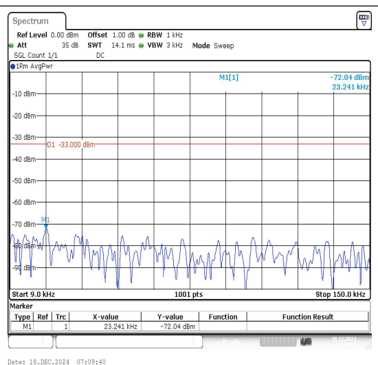
Band12_10MHz_16QAM_23060_1RB#0_0.009~0.15_0.009~0.15
