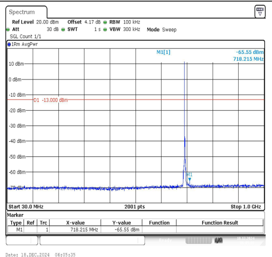
Band12_3MHz_16QAM_23025_1RB#0_30~1000_ 30~1000
