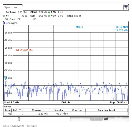
Band12_3MHz_16QAM_23025_1RB#0_0.009~0.1 5_0.009~0.15
