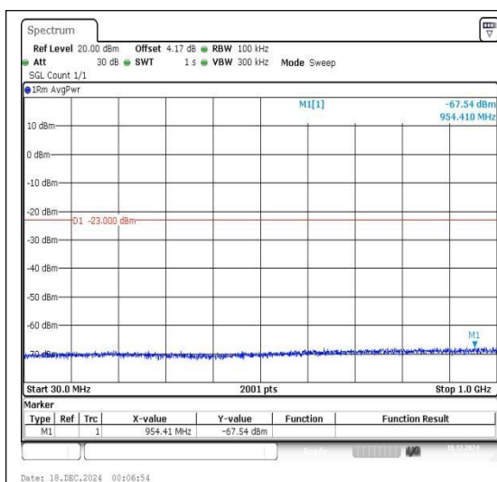
Band4_1.4MHz_QPSK_19957_1RB#0_30~1000_30~1000
