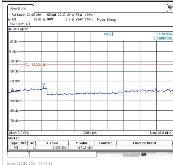
Band4_1.4MHz_QPSK_19957_1RB#0_3000~20000_00_3000~20000
