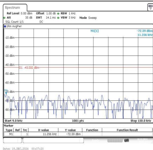
Band4_1.4MHz_16QAM_19957_1RB#0_0.009~0.15_15_0.009~0.15
