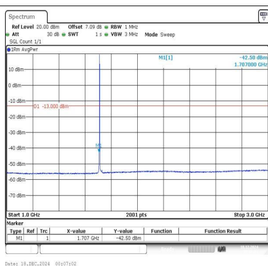
Band4_1.4MHz_QPSK_19957_1RB#0_1000~3000_0_1000~3000
