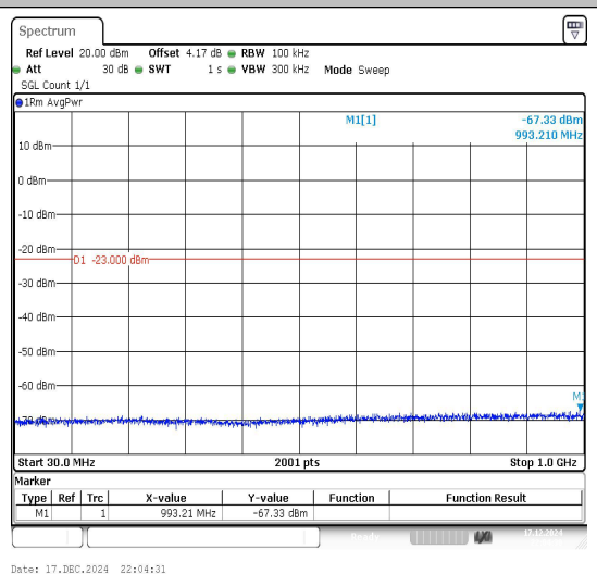
Band2_5MHz_16QAM_18900_1RB#0_30~1000_3 0~1000
