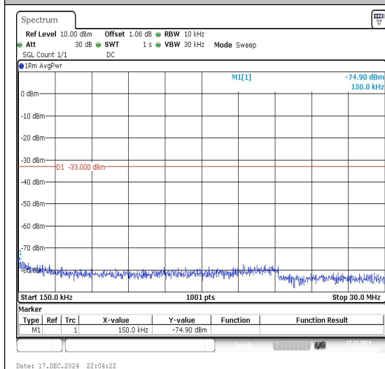
Band2_5MHz_16QAM_18900_1RB#0_0.15~30 0.15~30
