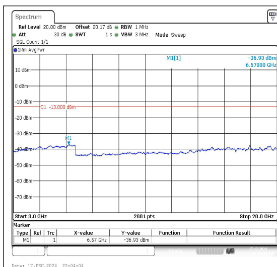
Band2_5MHz_QPSK_18900_1RB#0_3000~2000 0_3000~20000
