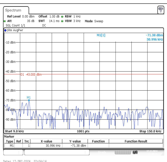
Band2_5MHz_16QAM_18900_1RB#0_0.009~0.15 _0.009~0.15
