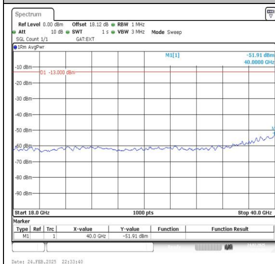
Band42_10MHz_QPSK_43040_1RB#0_18000~40000 0000_18000~40000
