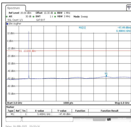
Band42_10MHz_QPSK_43040_1RB#0_3000~6000 00_3000~6000
