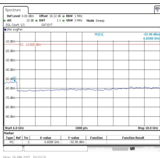
Band42_10MHz_QPSK_43040_1RB#0_6000~18000 00_6000~18000
