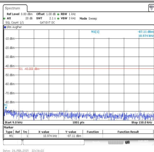
Band42_10MHz_16QAM_43040_1RB#0_0.009~0.15 15_0.009~0.15
