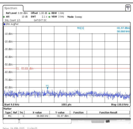
Band38_10MHz_16QAM_38200_1RB#0_0.009~0.15_0.009~0.15
