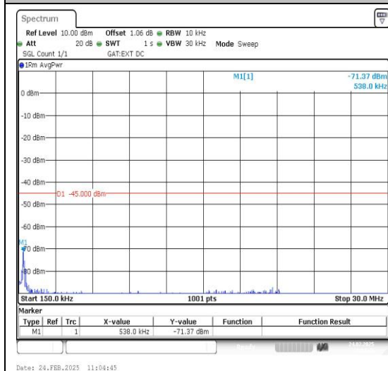
Band38_10MHz_QPSK_38200_1RB#0_0.15~30_0.15~30
