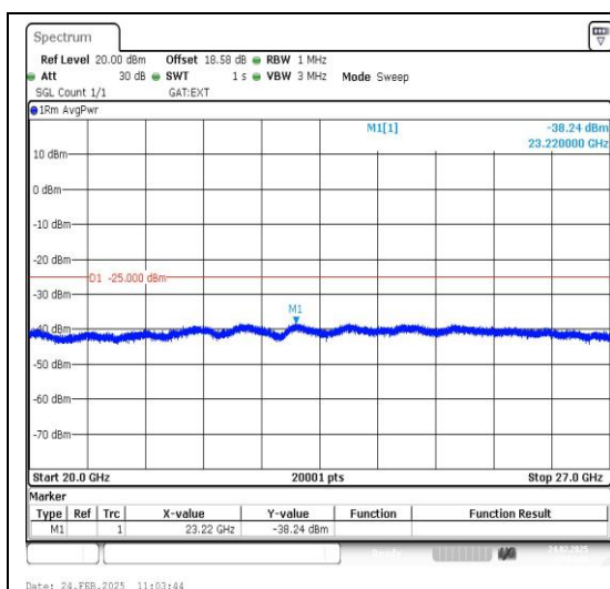
Band38_10MHz_QPSK_38200_1RB#0_20000~27000_20000~27000
