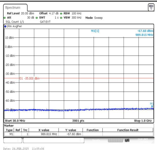
Band38_10MHz_16QAM_38200_1RB#0_30~1000_30~1000
