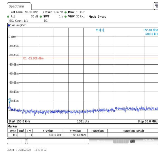
Band26_3MHz_16QAM_26915_1RB#0_0.15~30_0.15~30
