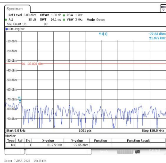
Band26_3MHz_16QAM_26915_1RB#0_0.009~0.15_0.009~0.15
