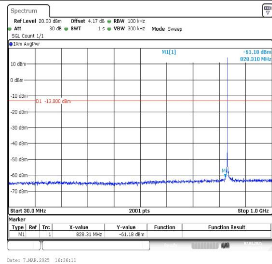
Band26_3MHz_16QAM_26915_1RB#0_30~1000_30~1000
