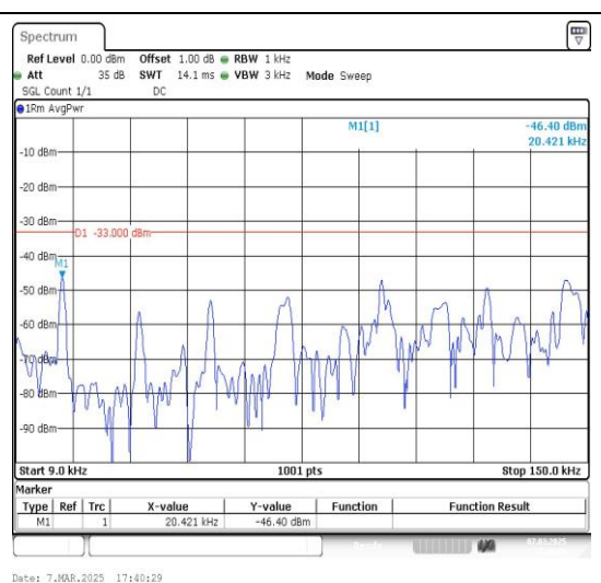
Band26_10MHz_16QAM_26990_1RB#0_0.009~0.15_0.009~0.15
