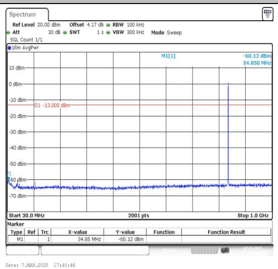
Band26_10MHz_16QAM_26990_1RB#0_30~1000_30~1000
