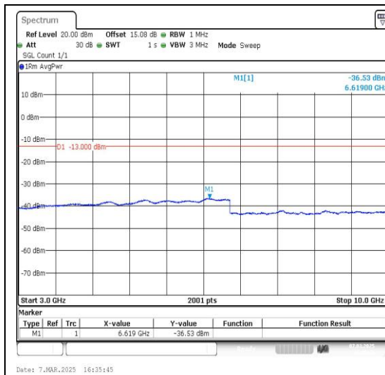
Band26_3MHz_QPSK_26915_1RB#0_3000~10000_3000~10000
