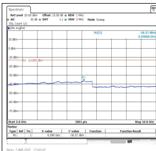
Band26_10MHz_QPSK_26990_1RB#0_3000~10000_3000~10000
