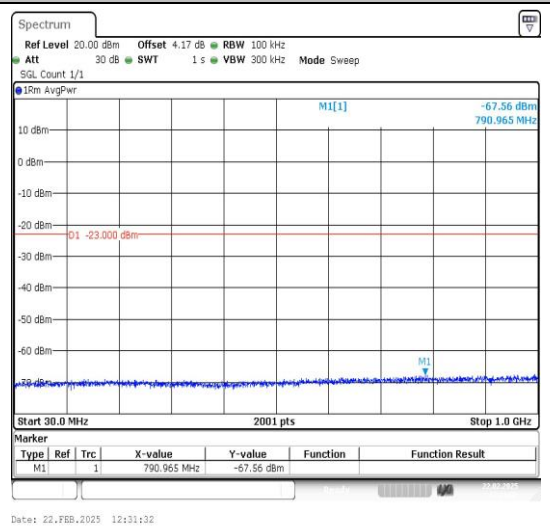
Band25_15MHz_16QAM_26615_1RB#0_30~1000_30~1000
