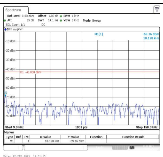
Band25_15MHz_16QAM_26615_1RB#0_0.009~0.15_0.009~0.15
