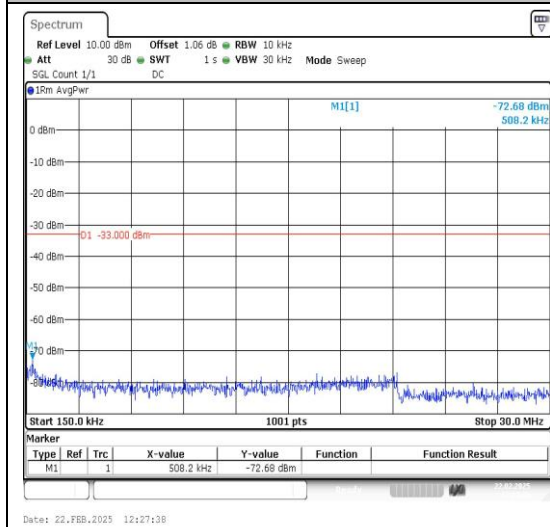
Band25_15MHz_16QAM_26115_1RB#0_0.15~30_0.15~30
