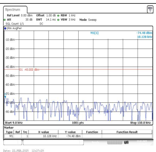
Band25_15MHz_16QAM_26115_1RB#0_0.009~0.15_0.009~0.15
