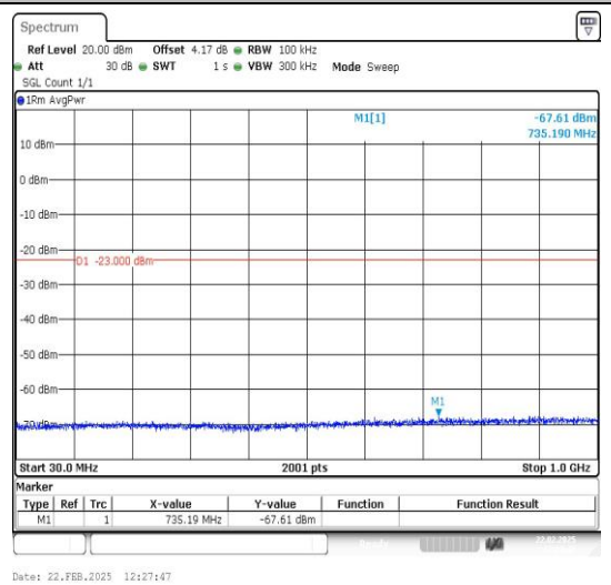
Band25_15MHz_16QAM_26115_1RB#0_30~1000_30~1000
