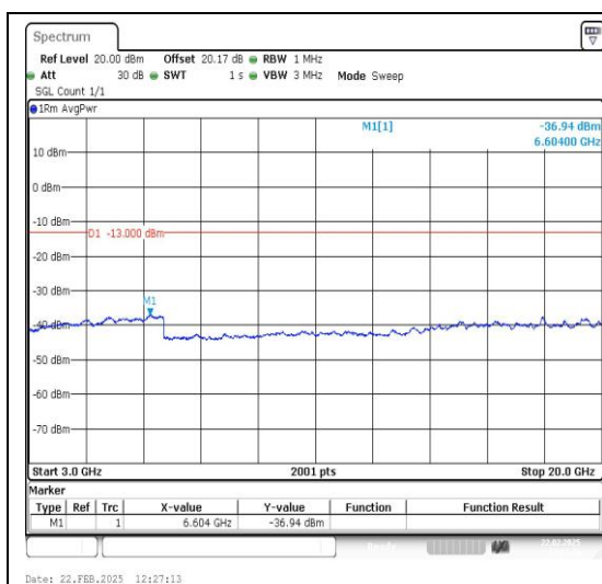
Band25_15MHz_QPSK_26115_1RB#0_3000~20000_3000~20000
