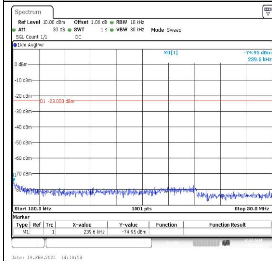
Band12_1.4MHz_16QAM_23095_1RB#0_0.15~30_0_0.15~30
