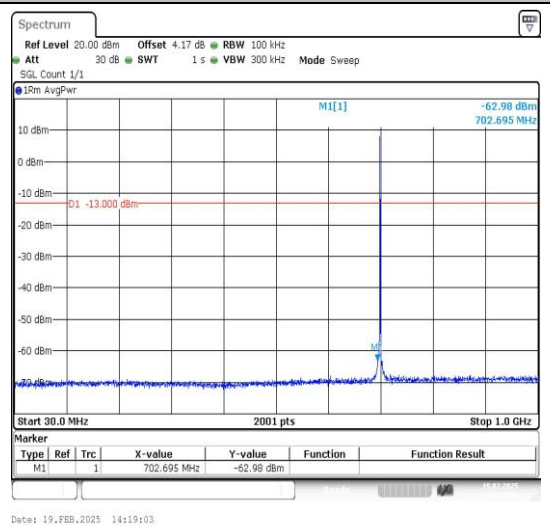
Band12_1.4MHz_16QAM_23095_1RB#0_30~1000_0_30~1000
