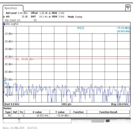
Band2_10MHz_16QAM_18900_1RB#0_0.009~0.15_0.009~0.15
