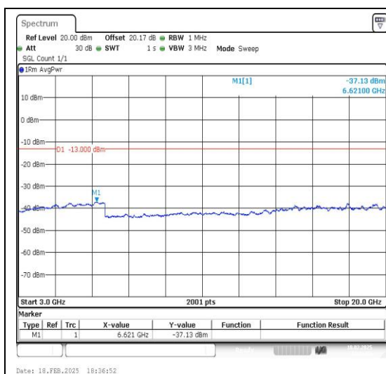
Band2_10MHz_QPSK_18900_1RB#0_3000~20000_3000~20000
