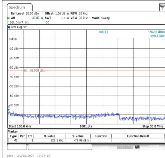
Band2_10MHz_16QAM_18900_1RB#0_0.15~30_0.15~30
