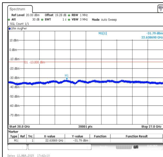
2-2-10MHz-15MHz-QPSK-QPSK-19005-19125-1 RB#49-0RB#0-20000~27000MHz-PASS
