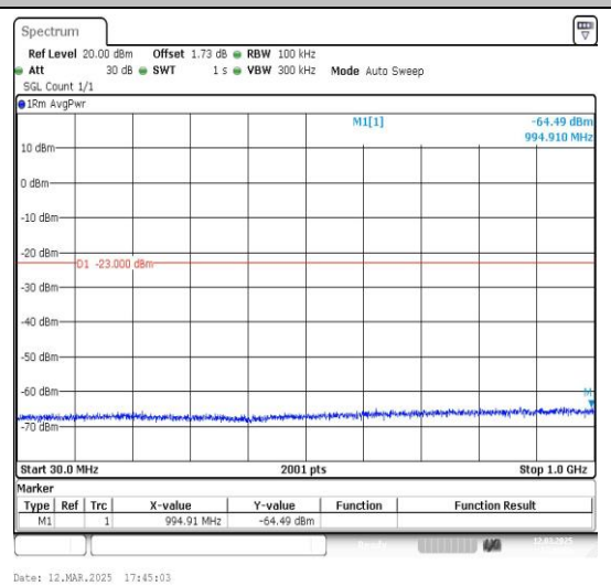
2-2-10MHz-15MHz-QPSK-QPSK-19005-19125-50 RB#0-75RB#0-30~1000MHz-PASS
