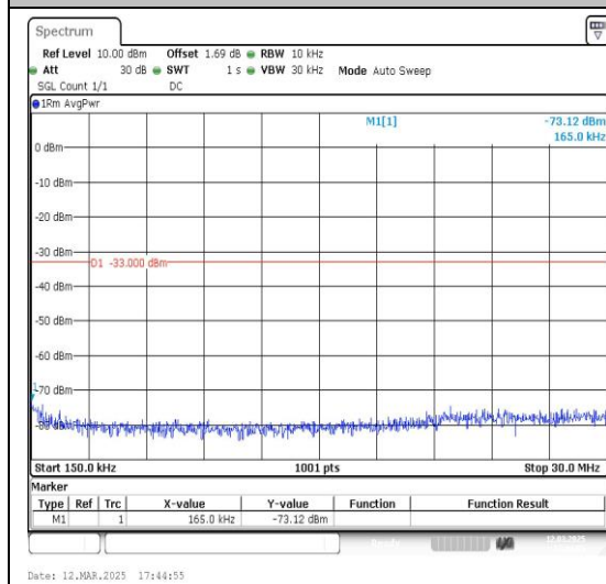
2-2-10MHz-15MHz-QPSK-QPSK-19005-19125-5 0RB#0-75RB#0-0.15~30MHz-PASS
