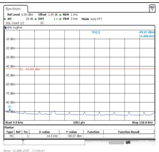
2-2-10MHz-15MHz-QPSK-QPSK-19005-19125-50 RB#0-75RB#0-0.009~0.15MHz-PASS
