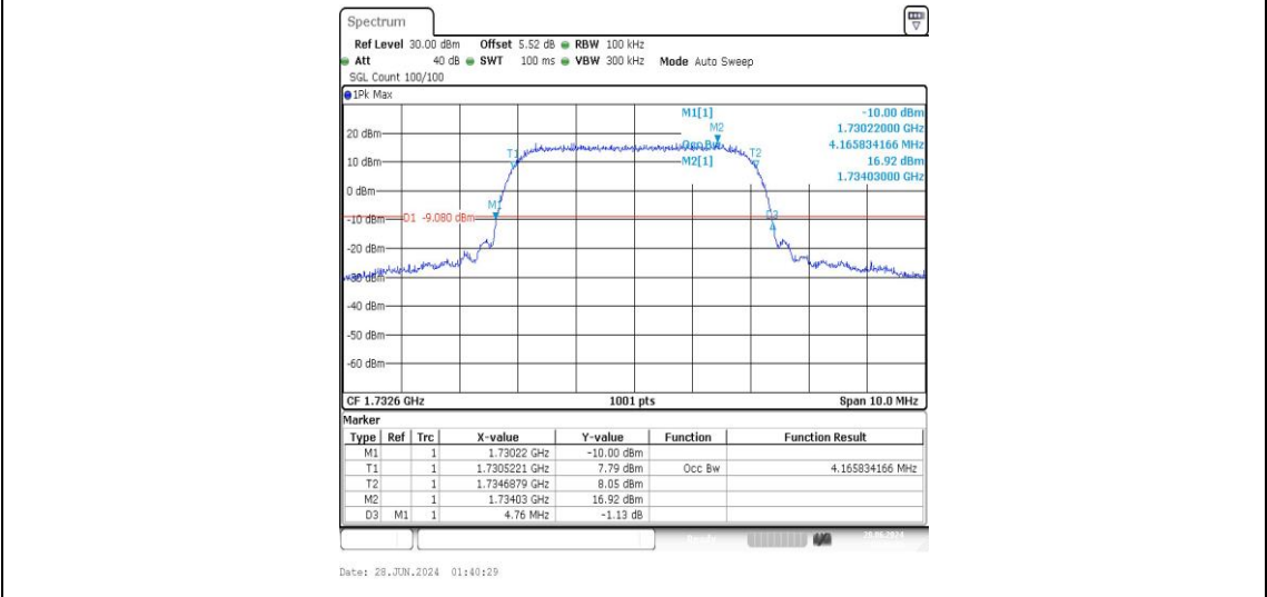
Band4-1413-1-PASS
