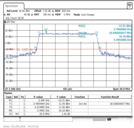
Band41-20MHz-16QAM-39750-100RB#0-PASS
