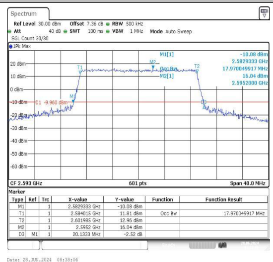
Band41-20MHz-16QAM-40620-100RB#0-PASS
