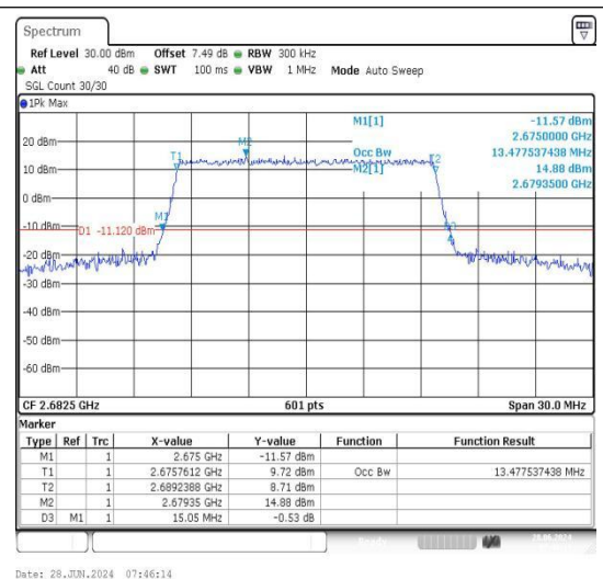
Band41-15MHz-16QAM-41515-75RB#0-PASS
