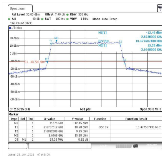
Band41-15MHz-QPSK-41515-75RB#0-PASS
