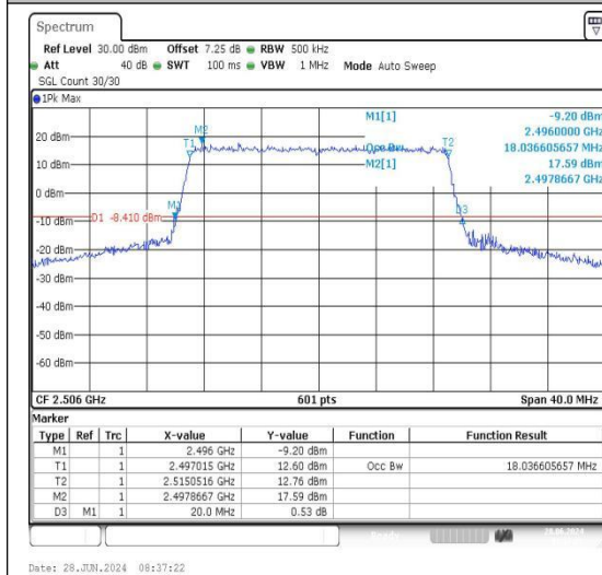
Band41-20MHz-QPSK-39750-100RB#0-PASS
