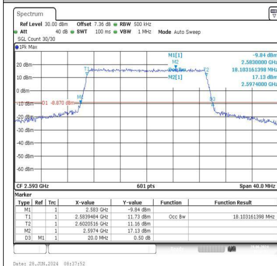
Band41-20MHz-QPSK-40620-100RB#0-PASS
