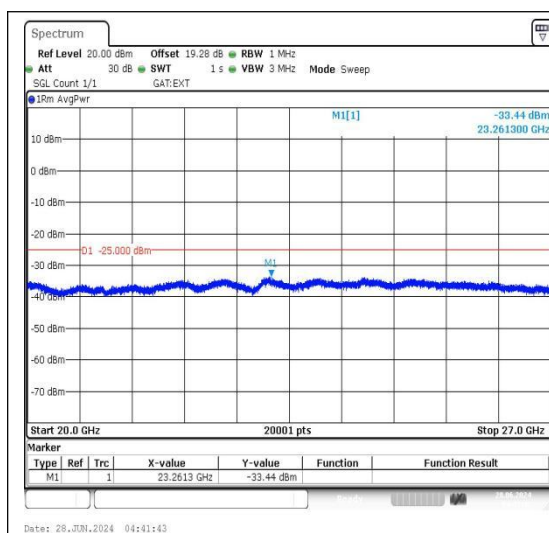
Band38_15MHz_QPSK_38175_1RB#0_20000~27000
