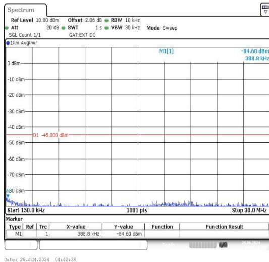
Band38_15MHz_QPSK_38175_1RB#0_0.15~30
