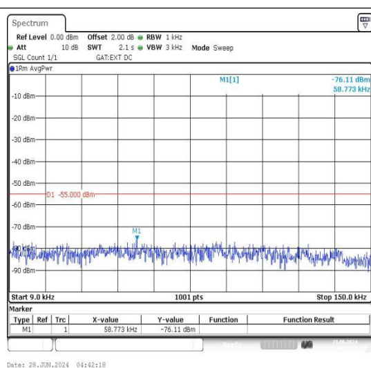
Band38_15MHz_16QAM_38175_1RB#0_0.009~0.15
