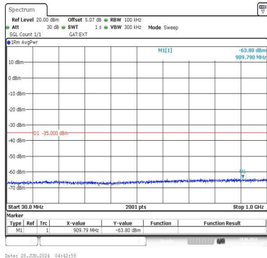
Band38_15MHz_16QAM_38175_1RB#0_30~1000
